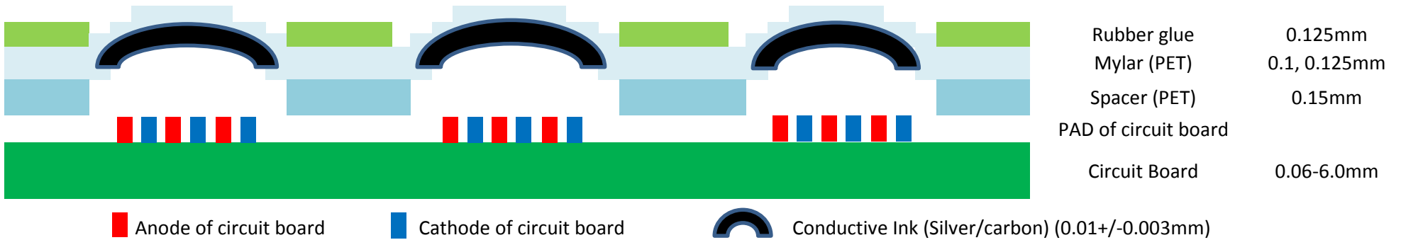
Polydome with glue stack up
