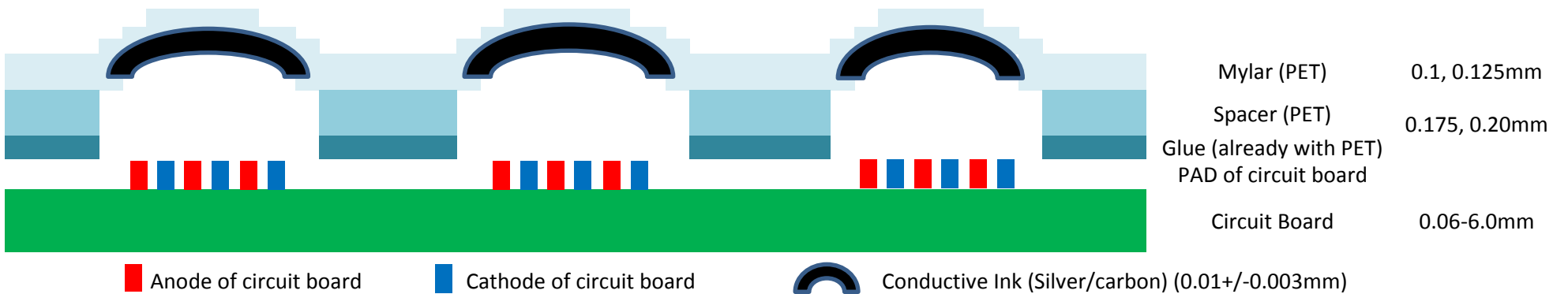
Polydome with glue stack up
