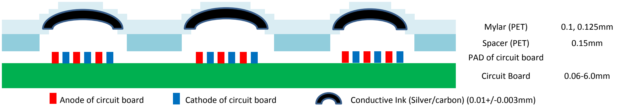
Polydome with rubber glue stack up
