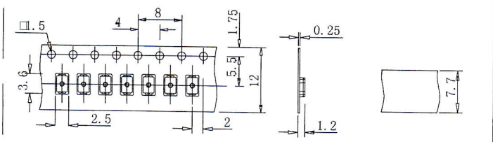
SCALE 1.2:1 CARRIER TAPE
